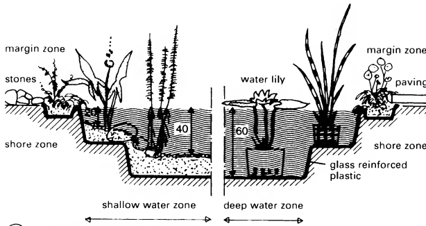
② A suitable prefabricated pond
